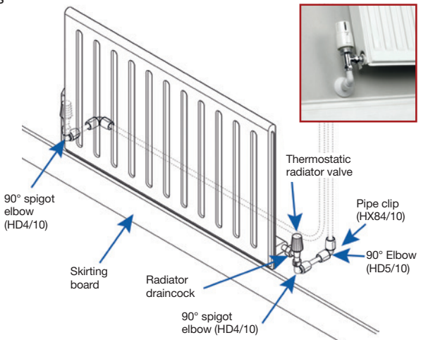
Figure 52: Radiator pipework in 10mm Hep 2 O within dry lined walls
