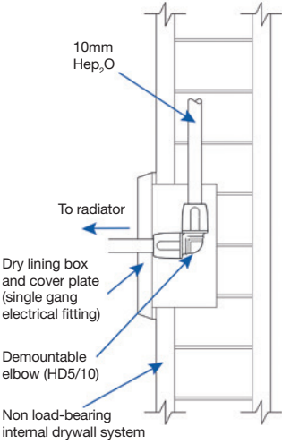
Figure 57: Radiator connection using 10mm Hep 2 O and a dry lining box within a drywall
