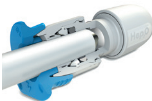
Figure 20: Cut-away drawing of HepKey™
