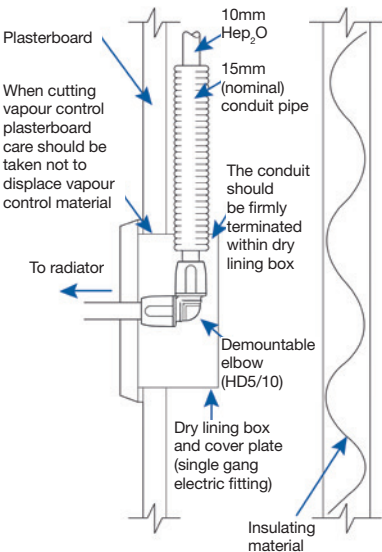
Figure 58: Radiator connection using 10mm Hep 2 O within timber or steel framed external wall
