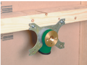
Figure 50: Installation of HX102 terminal fitting plate and HX101/15, 15mm conduit terminal
